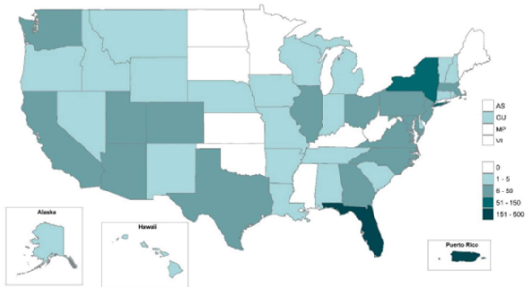
Figure 1. Dengue cases reported to ArboNET — United States, 2023 (as of October 4, 2023).
